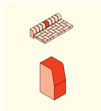
Fig 7 Kerb
