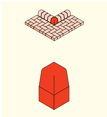
Fig 7 Kerb 90° External Return
